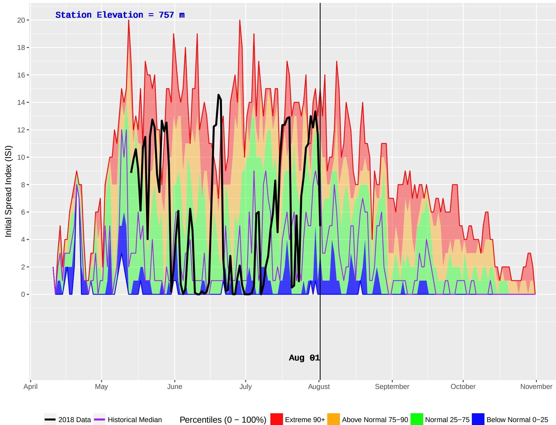
DOWNIE (905) : Historical (2005–2016) and Current (2018) Daily Initial Spread Index (ISI)
