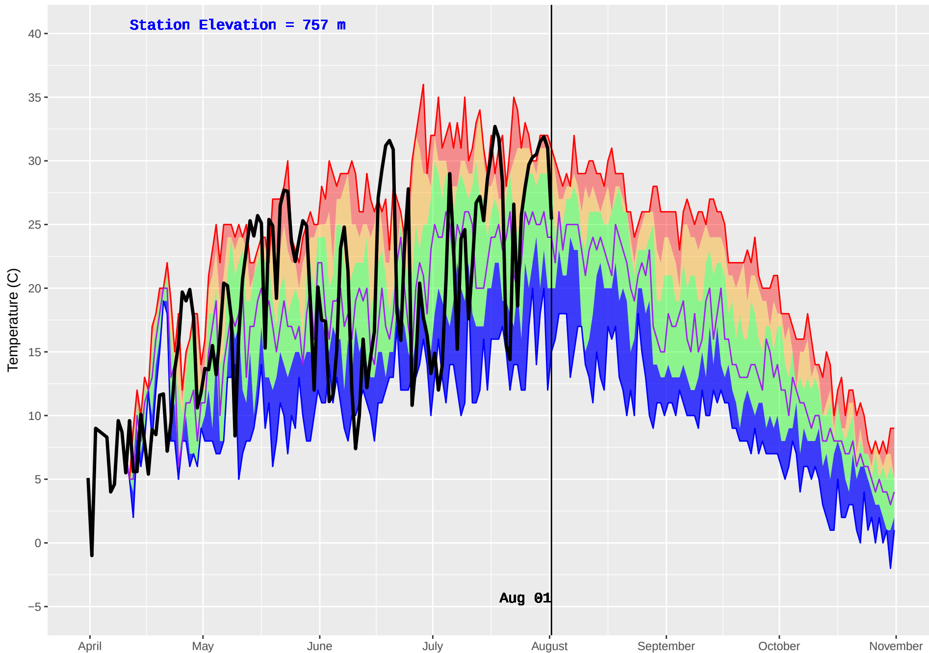
DOWNIE (905) : Historical (2005–2016) and Current (2018) Daily Temperature
