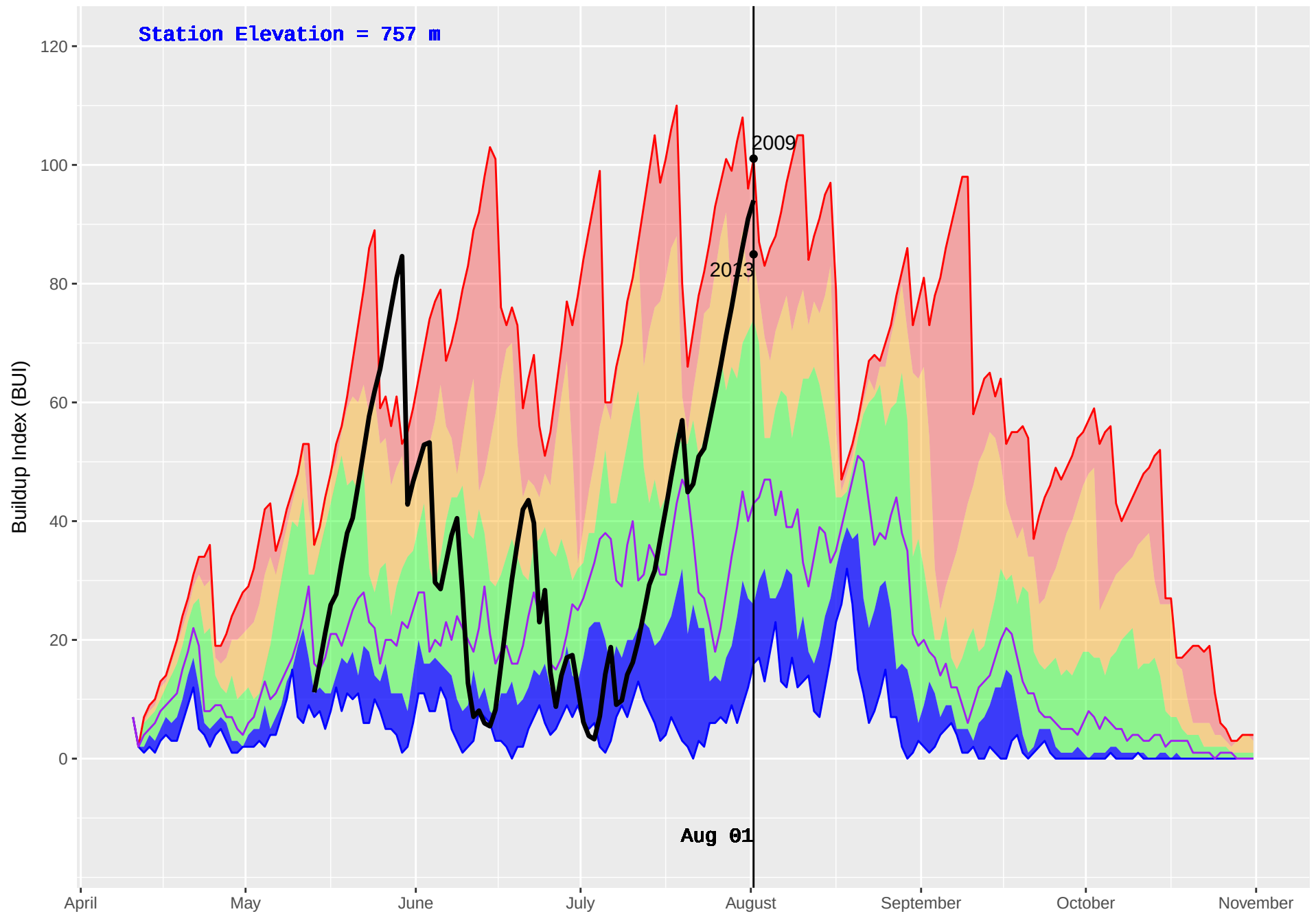
DOWNIE (905) : Historical (2005–2016) and Current (2018) Daily Buildup Index (BUI)
