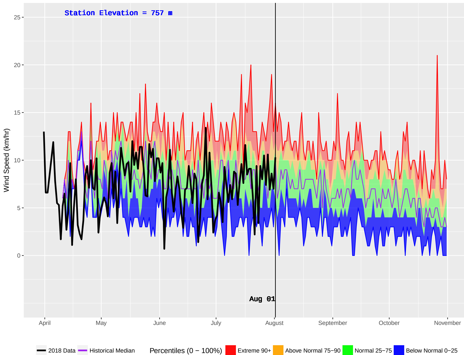
DOWNIE (905) : Historical (2005–2016) and Current (2018) Daily Wind Speed
